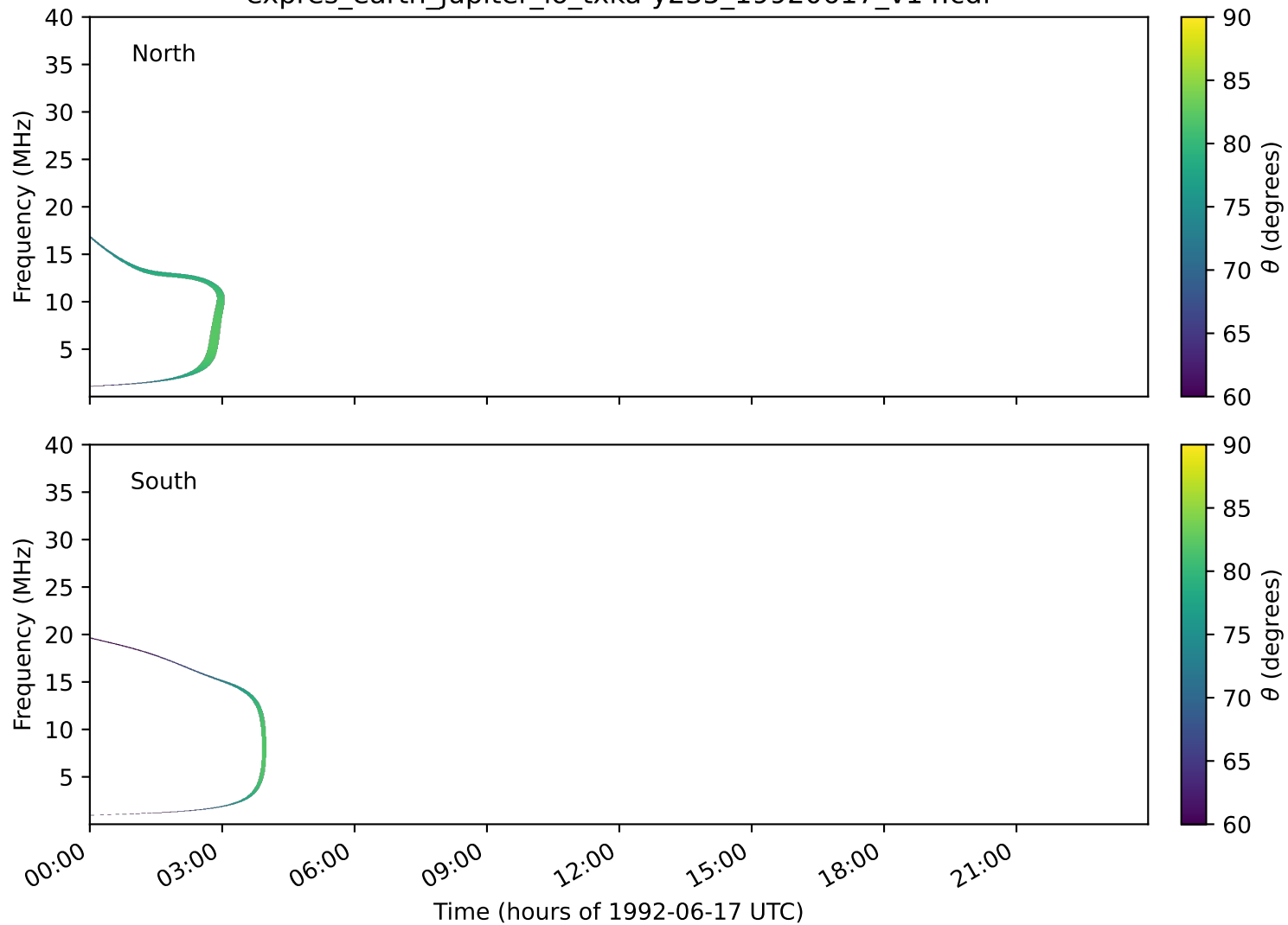
expres_earth_jupiter_io_txka-y235_19920617_v14.cdf
