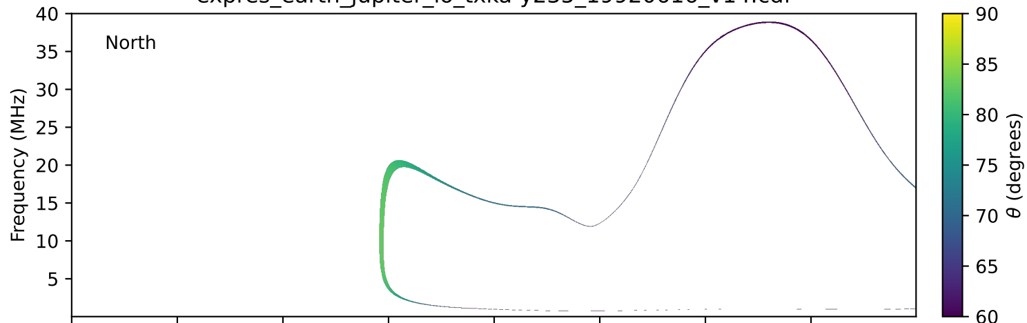
expres_earth_jupiter_io_txka-y235_19920616_v14.cdf
