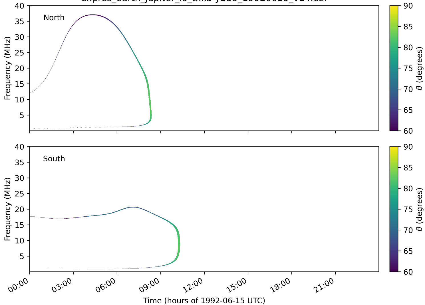
expres_earth_jupiter_io_txka-y235_19920615_v14.cdf
