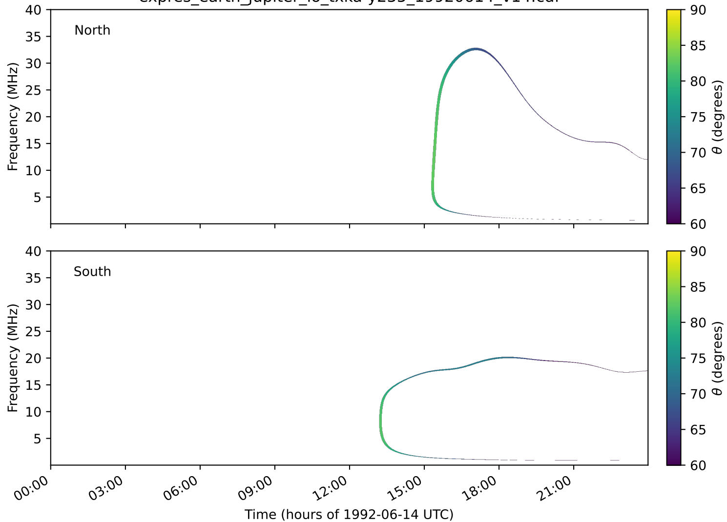
expres_earth_jupiter_io_txka-y235_19920614_v14.cdf
