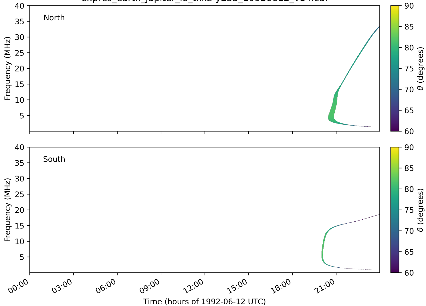
expres_earth_jupiter_io_txka-y235_19920612_v14.cdf
