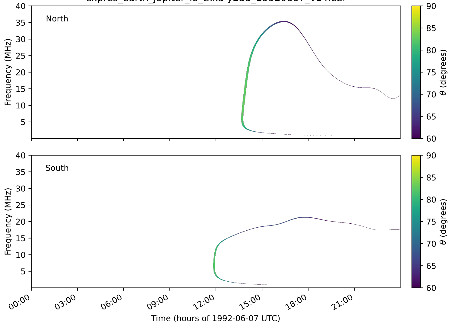
expres_earth_jupiter_io_txka-y235_19920607_v14.cdf
