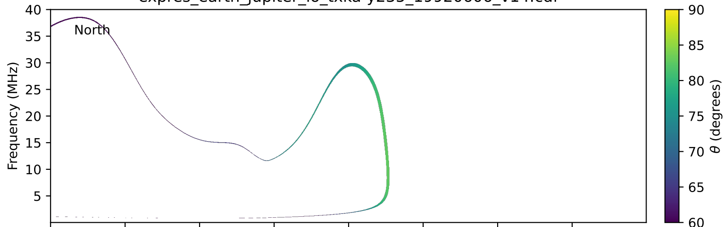
expres_earth_jupiter_io_txka-y235_19920606_v14.cdf
