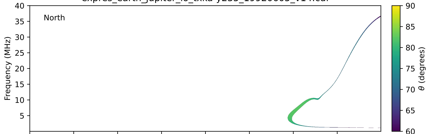
expres_earth_jupiter_io_txka-y235_19920605_v14.cdf
