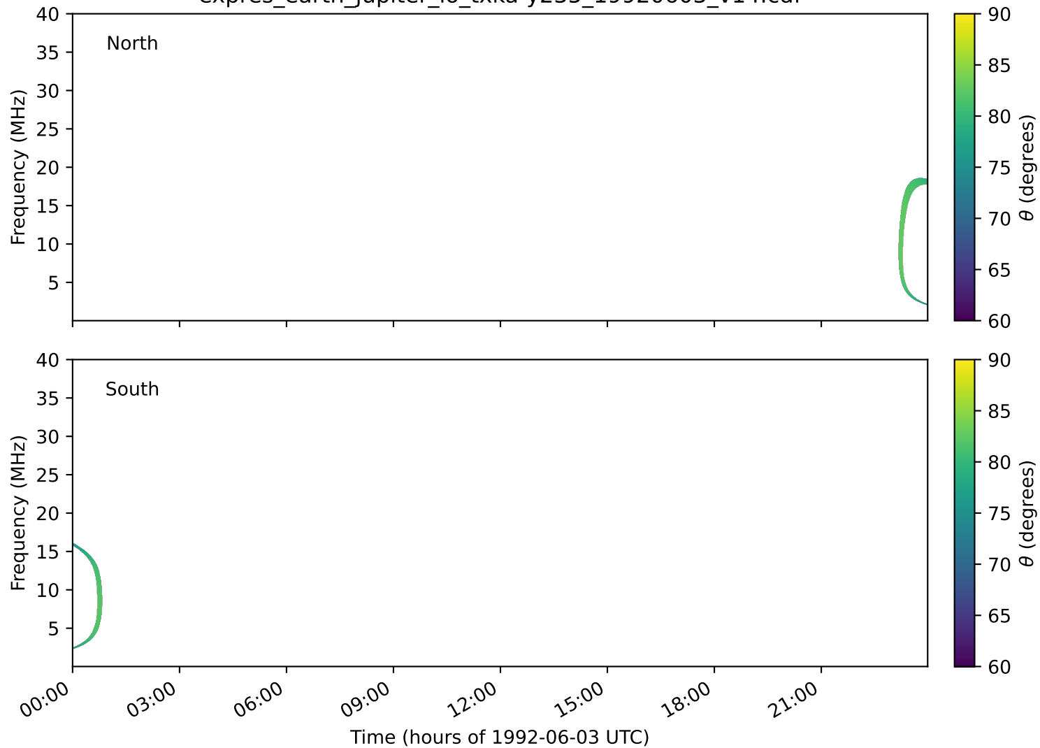
expres_earth_jupiter_io_txka-y235_19920603_v14.cdf
