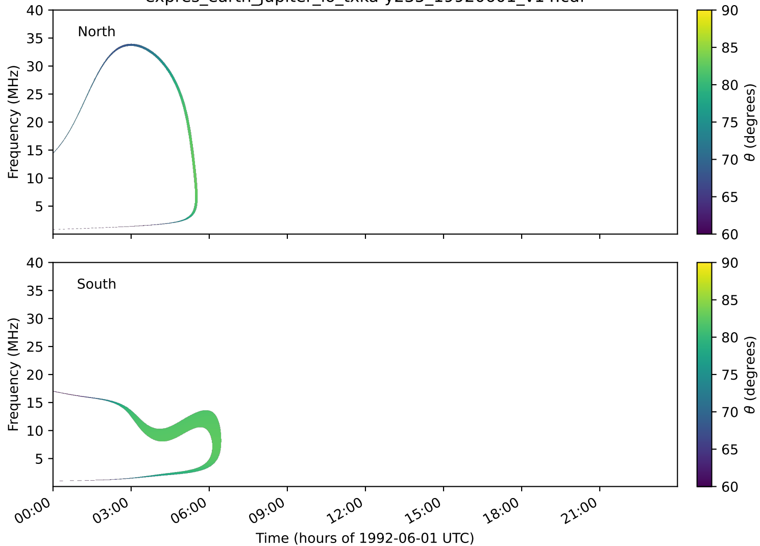
expres_earth_jupiter_io_txka-y235_19920601_v14.cdf
