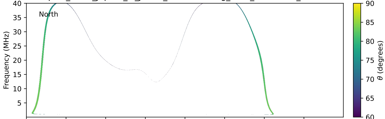
expres_earth_jupiter_io_jrm33_lossc-wid1deg_3kev_19920627_v11.cdf
