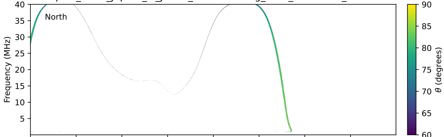
expres_earth_jupiter_io_jrm33_lossc-wid1deg_3kev_19920620_v11.cdf
