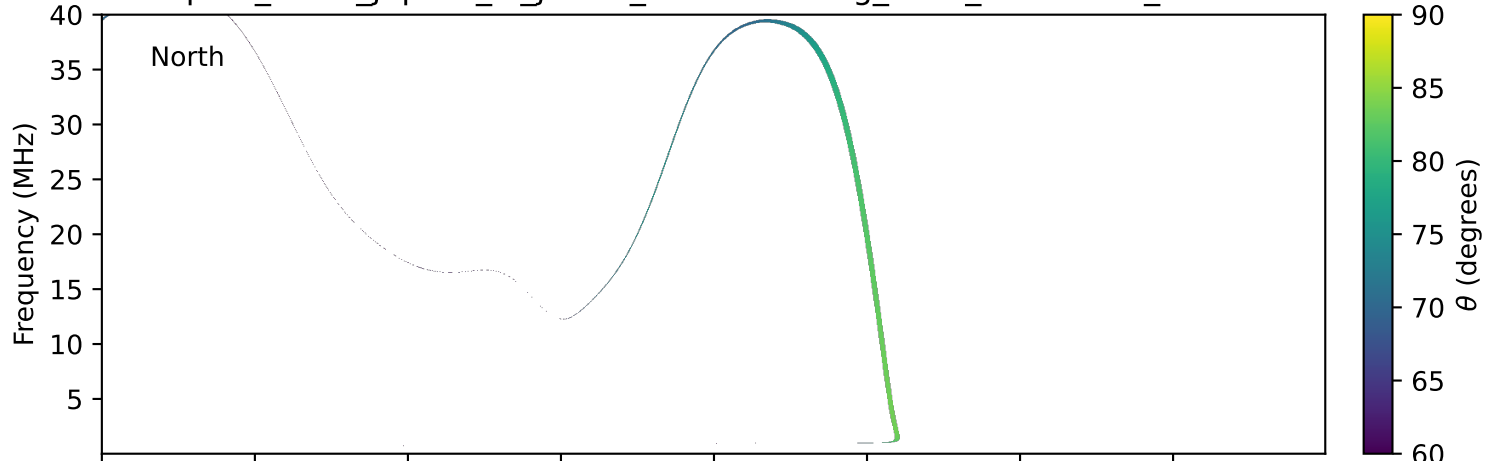
expres_earth_jupiter_io_jrm33_lossc-wid1deg_3kev_19920613_v11.cdf
