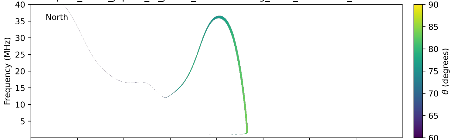
expres_earth_jupiter_io_jrm33_lossc-wid1deg_3kev_19920606_v11.cdf
