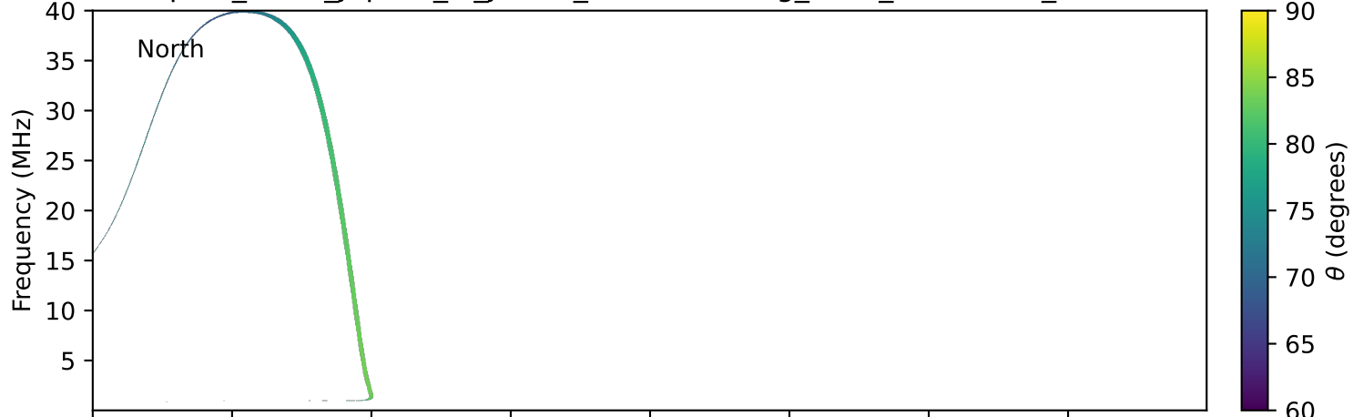
expres_earth_jupiter_io_jrm33_lossc-wid1deg_3kev_19920601_v11.cdf
