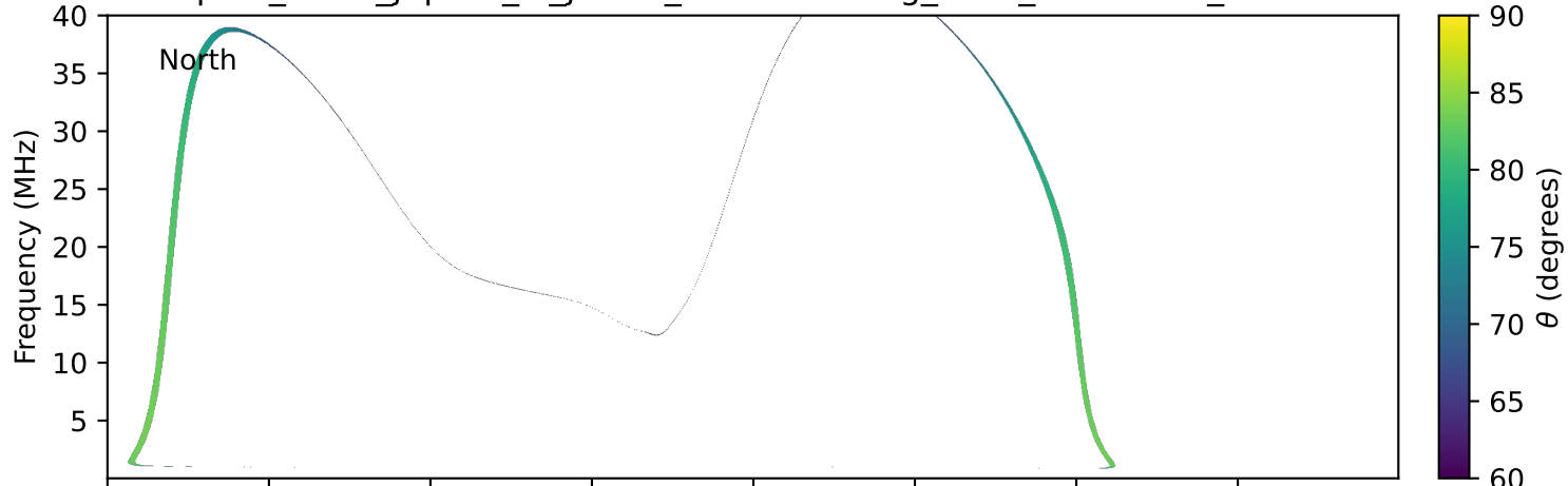
expres_earth_jupiter_io_jrm09_lossc-wid1deg_3kev_19920627_v11.cdf
