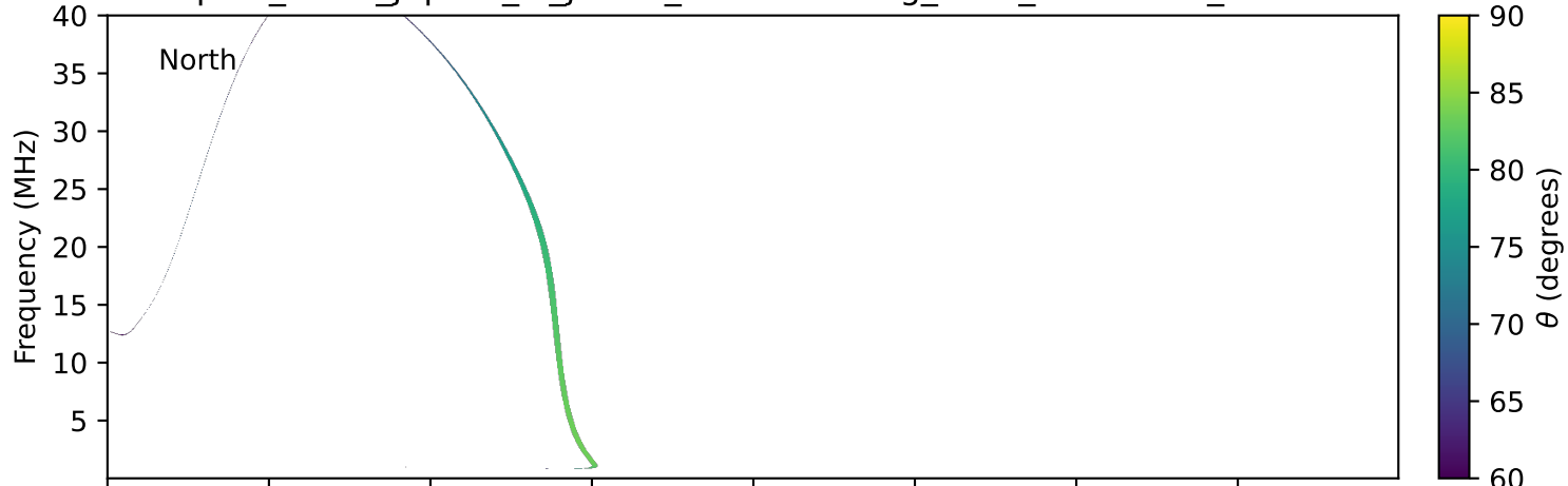
expres_earth_jupiter_io_jrm09_lossc-wid1deg_3kev_19920615_v11.cdf
