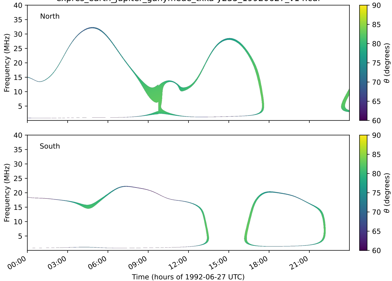
expres_earth_jupiter_ganymede_txka-y235_19920627_v14.cdf
