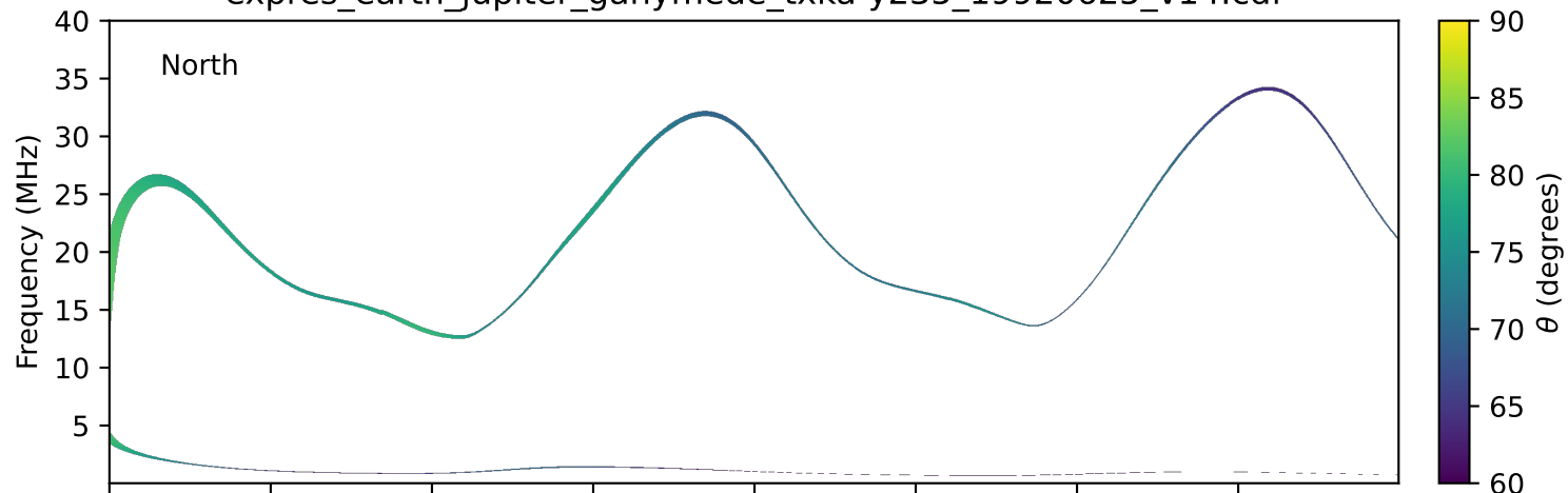
expres_earth_jupiter_ganymede_txka-y235_19920625_v14.cdf
