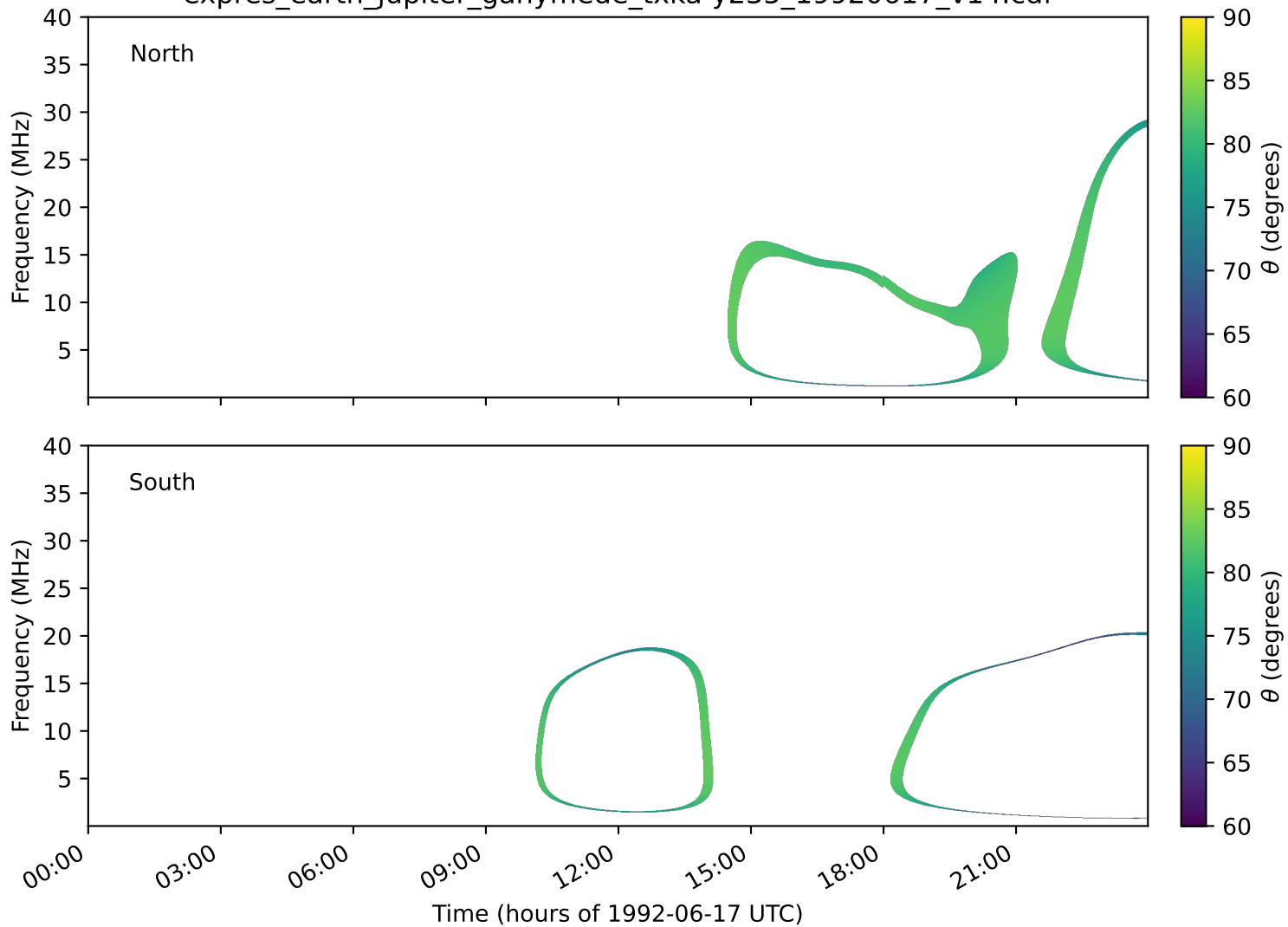
expres_earth_jupiter_ganymede_txka-y235_19920617_v14.cdf
