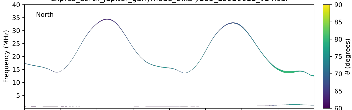
expres_earth_jupiter_ganymede_txka-y235_19920612_v14.cdf
