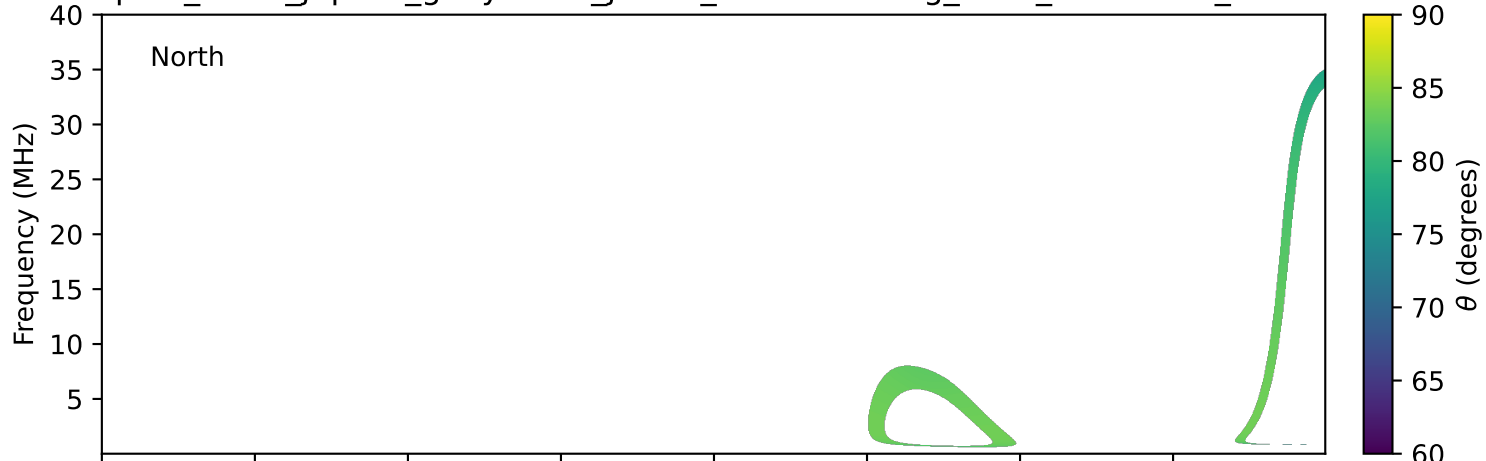
expres_earth_jupiter_ganymede_jrm33_lossc-wid1deg_3kev_19920617_v11.cdf
