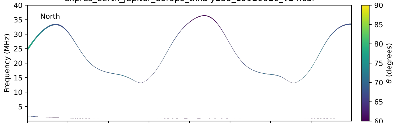
expres_earth_jupiter_europa_txka-y235_19920620_v14.cdf
