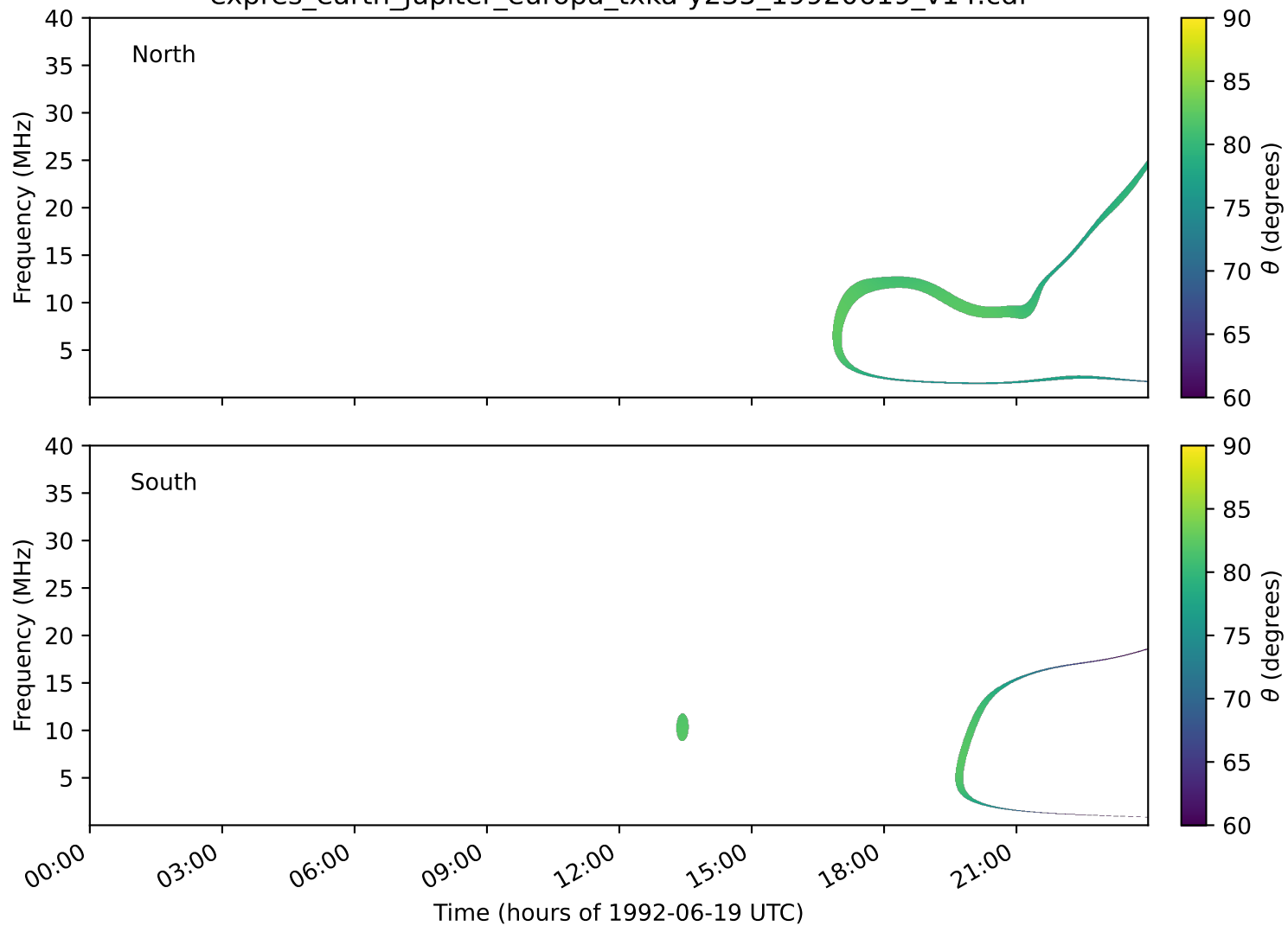
expres_earth_jupiter_europa_txka-y235_19920619_v14.cdf
