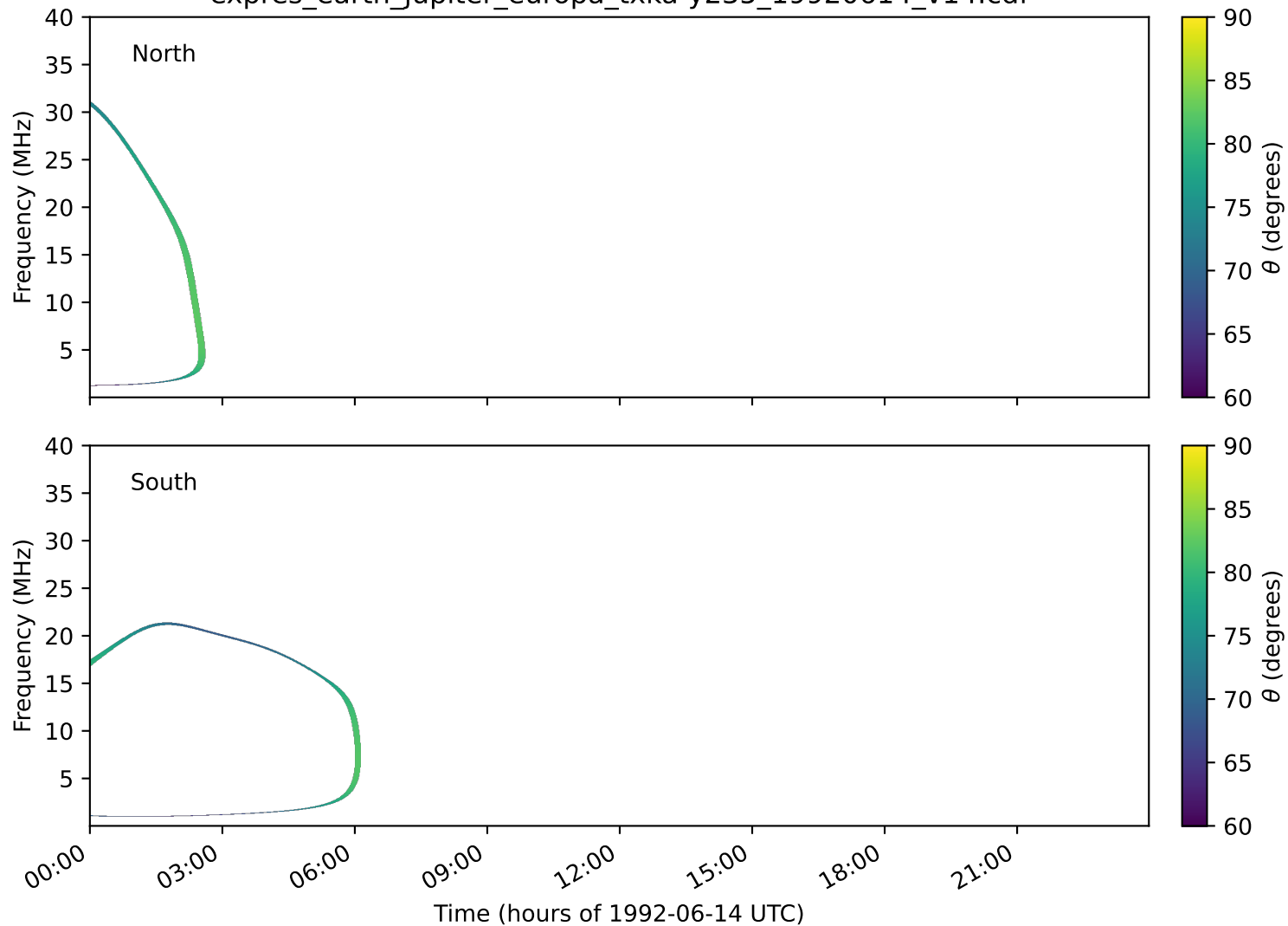
expres_earth_jupiter_europa_txka-y235_19920614_v14.cdf
