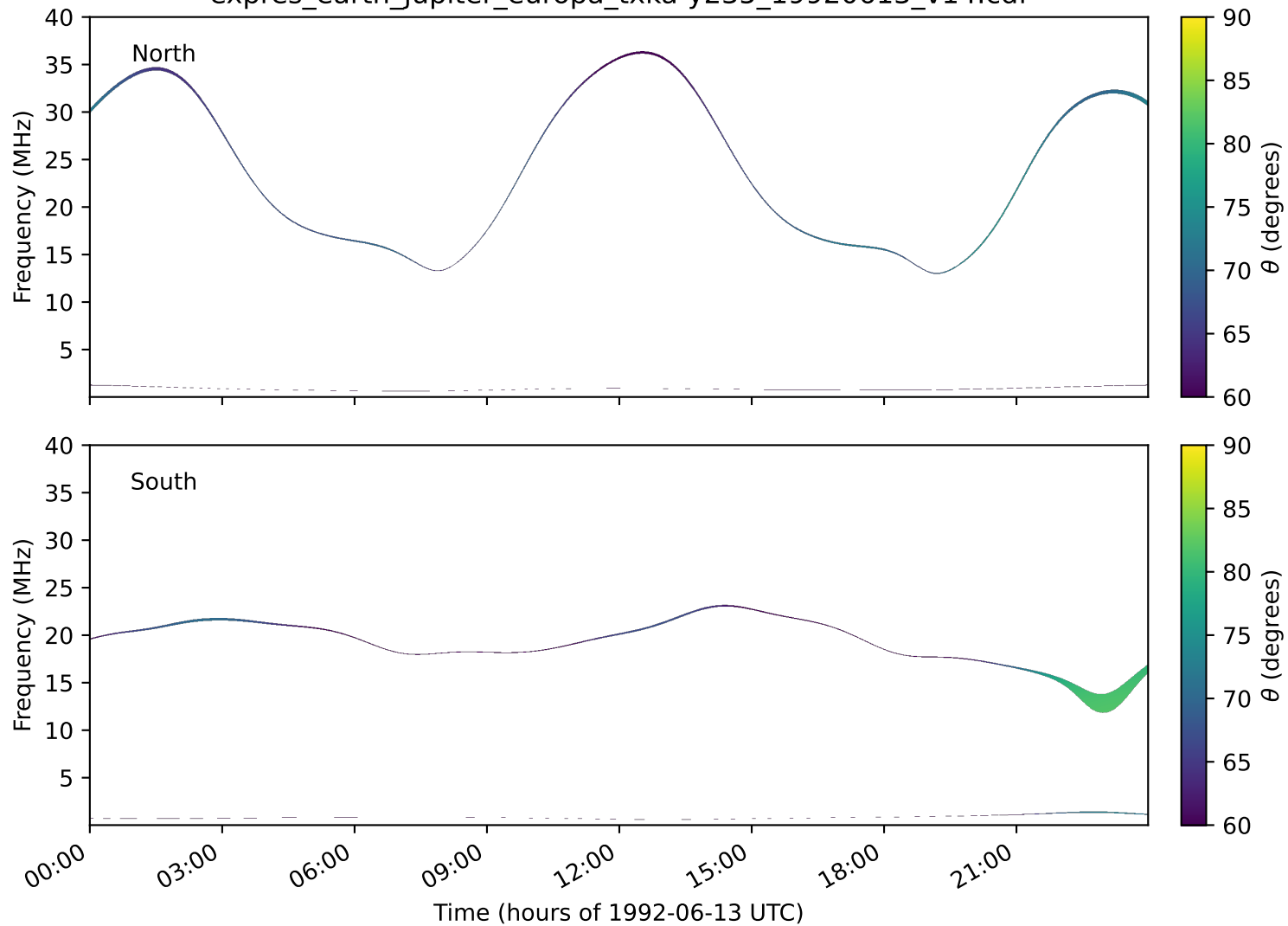
expres_earth_jupiter_europa_txka-y235_19920613_v14.cdf
