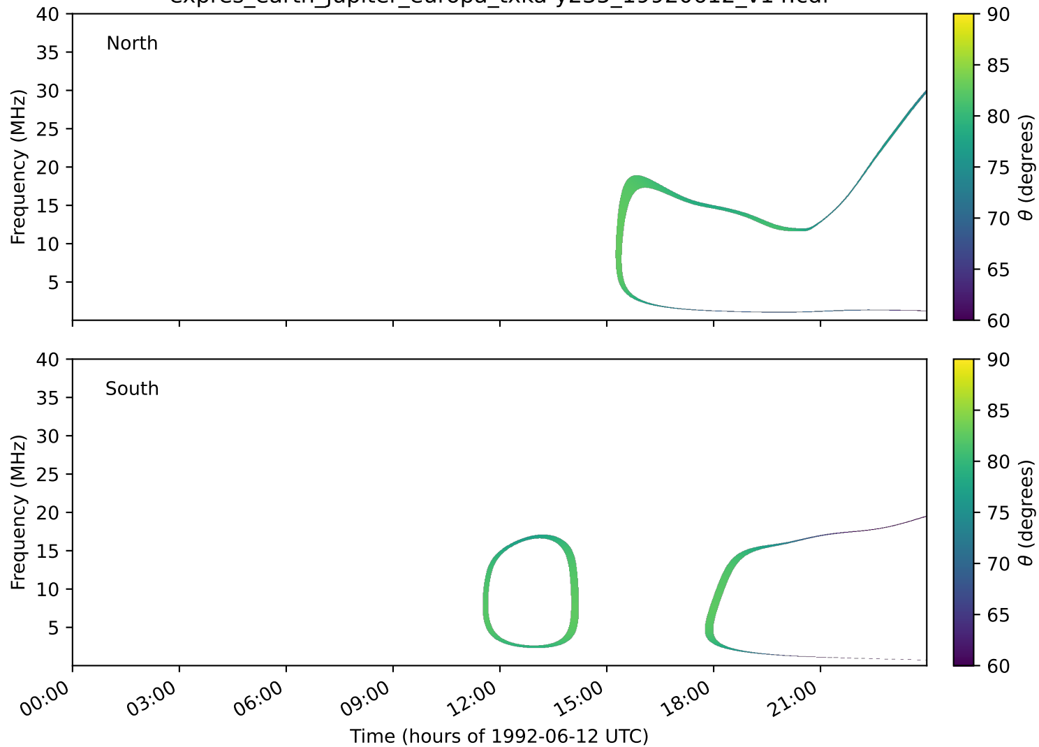
expres_earth_jupiter_europa_txka-y235_19920612_v14.cdf
