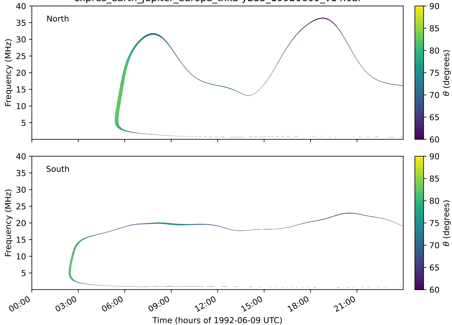
expres_earth_jupiter_europa_txka-y235_19920609_v14.cdf
