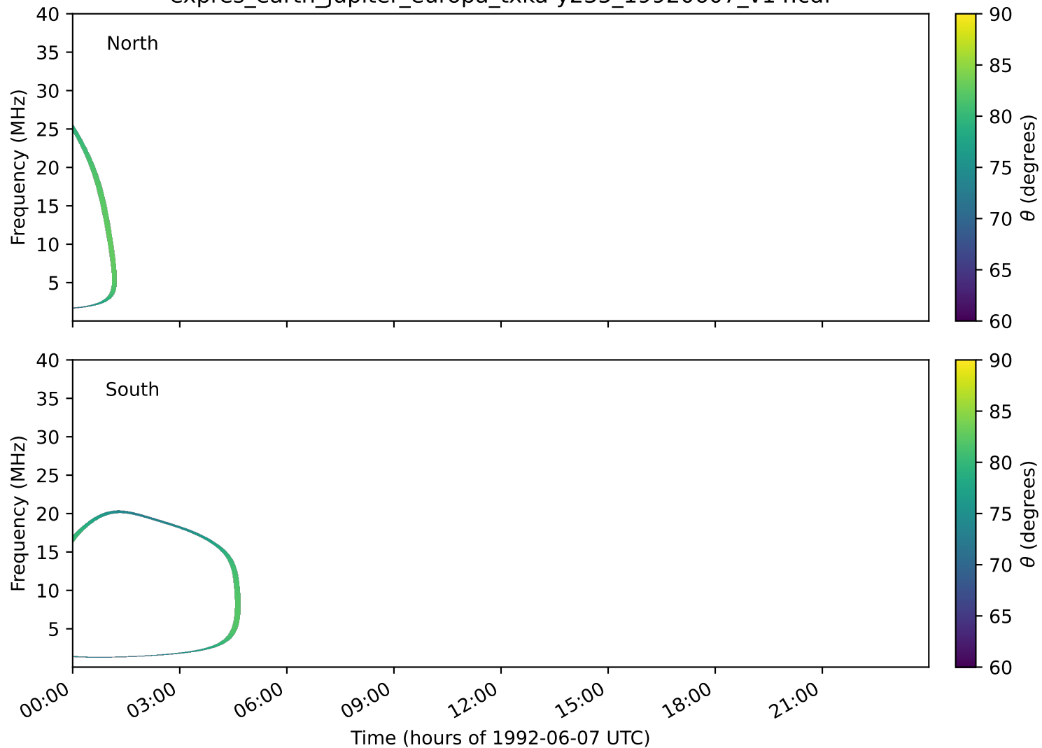
expres_earth_jupiter_europa_txka-y235_19920607_v14.cdf
