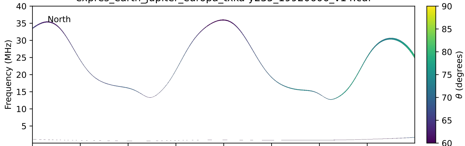
expres_earth_jupiter_europa_txka-y235_19920606_v14.cdf
