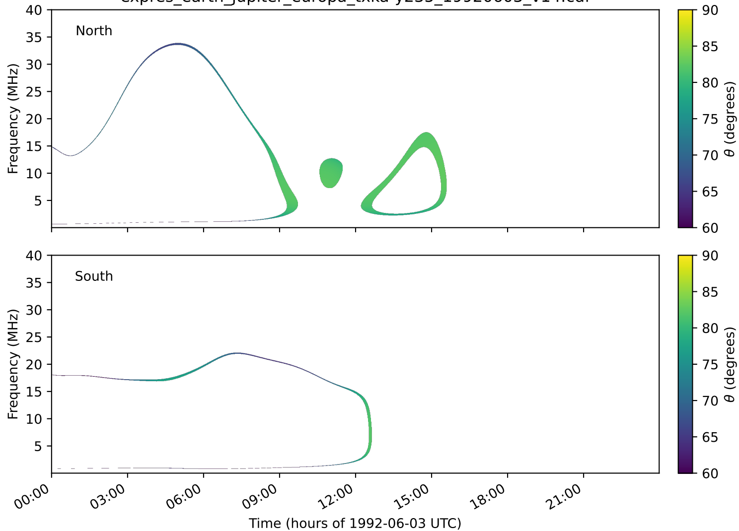
expres_earth_jupiter_europa_txka-y235_19920603_v14.cdf
