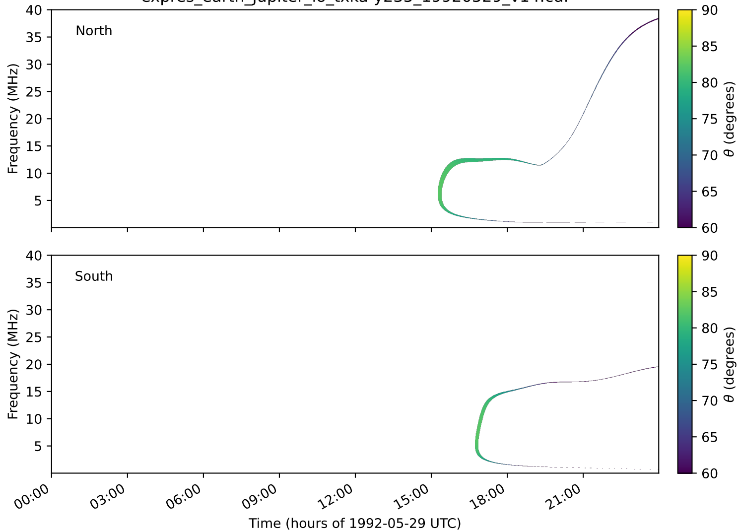
expres_earth_jupiter_io_txka-y235_19920529_v14.cdf
