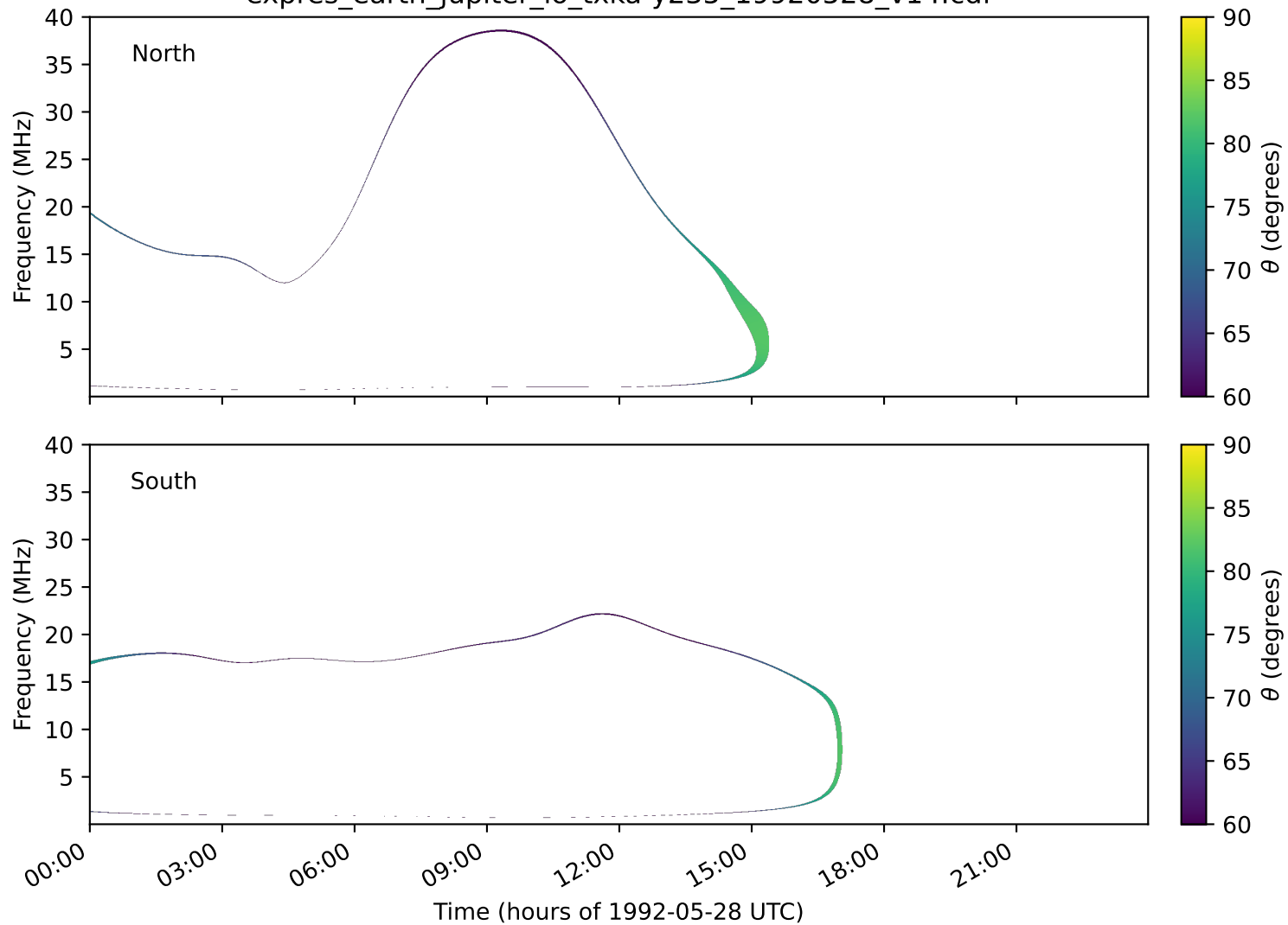
expres_earth_jupiter_io_txka-y235_19920528_v14.cdf
