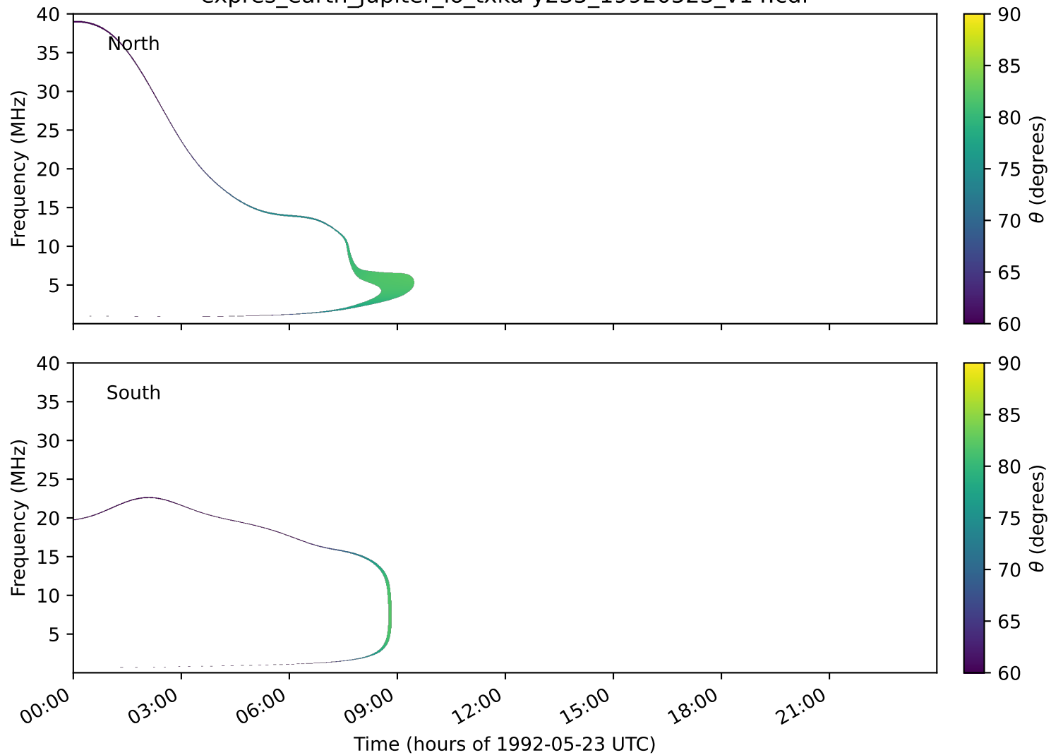
expres_earth_jupiter_io_txka-y235_19920523_v14.cdf
