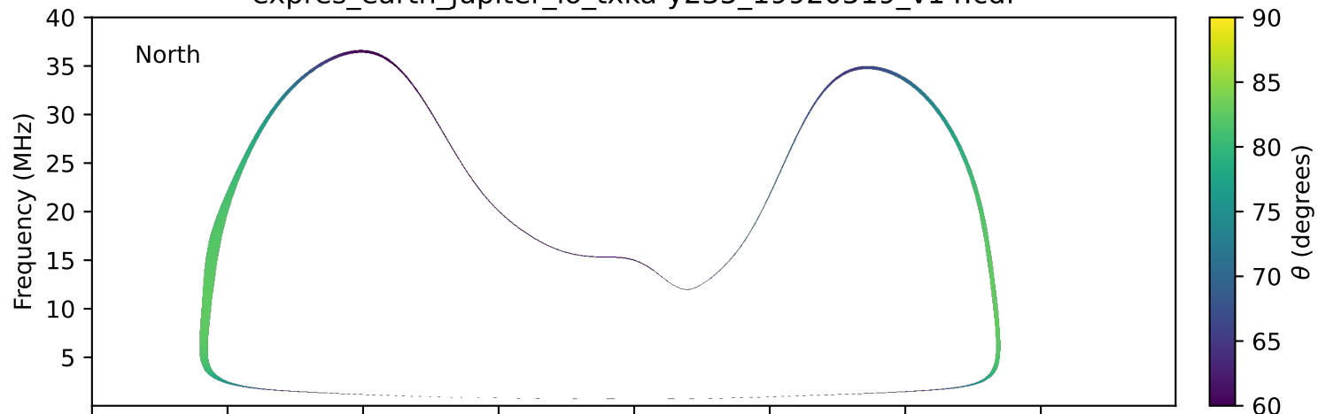
expres_earth_jupiter_io_txka-y235_19920519_v14.cdf
