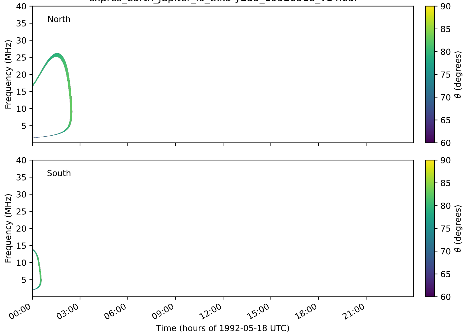
expres_earth_jupiter_io_txka-y235_19920518_v14.cdf
