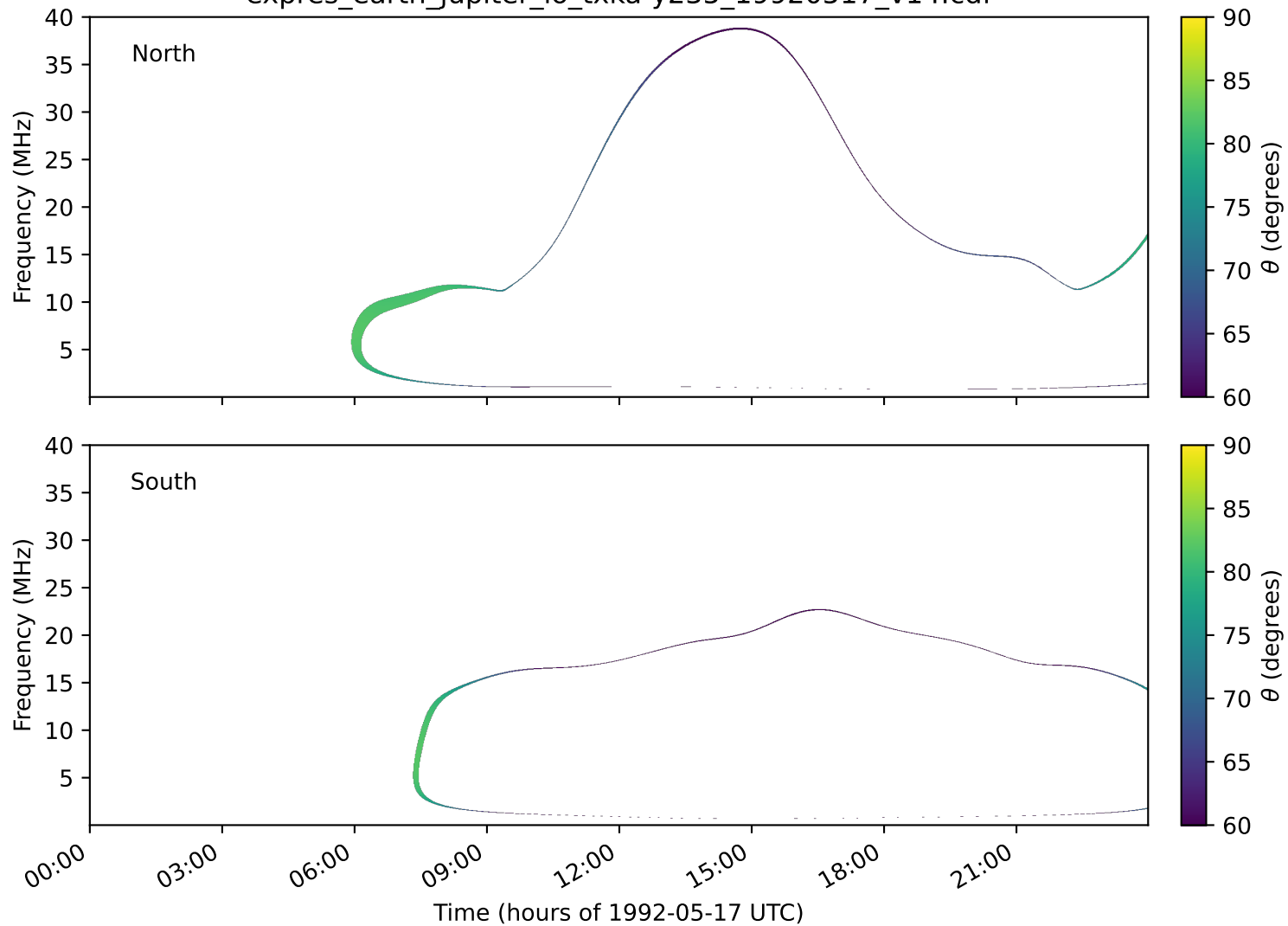
expres_earth_jupiter_io_txka-y235_19920517_v14.cdf
