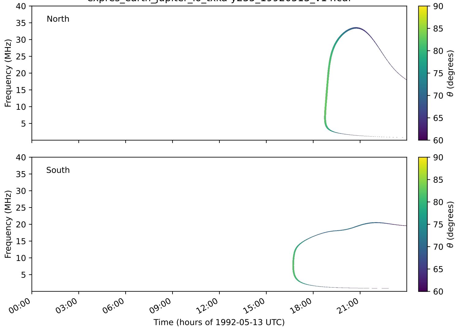
expres_earth_jupiter_io_txka-y235_19920513_v14.cdf
