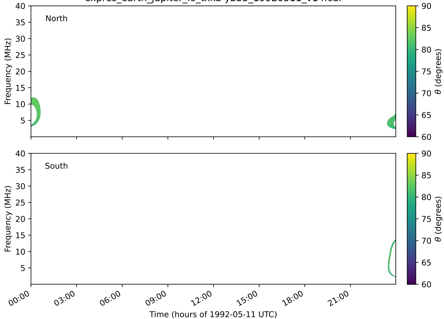
expres_earth_jupiter_io_txka-y235_19920511_v14.cdf
