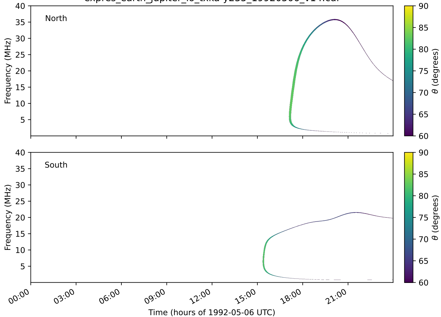
expres_earth_jupiter_io_txka-y235_19920506_v14.cdf
