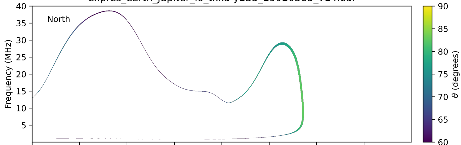
expres_earth_jupiter_io_txka-y235_19920505_v14.cdf
