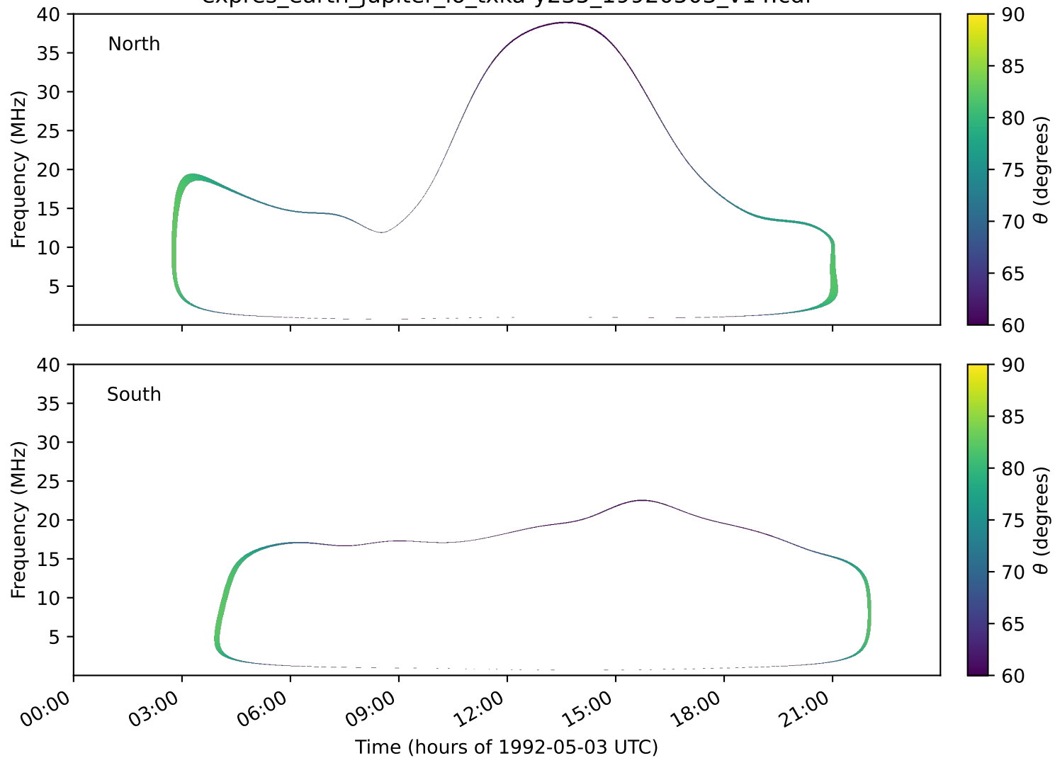
expres_earth_jupiter_io_txka-y235_19920503_v14.cdf
