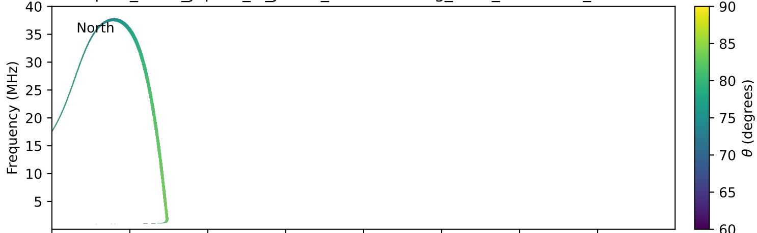
expres_earth_jupiter_io_jrm33_lossc-wid1deg_3kev_19920525_v11.cdf
