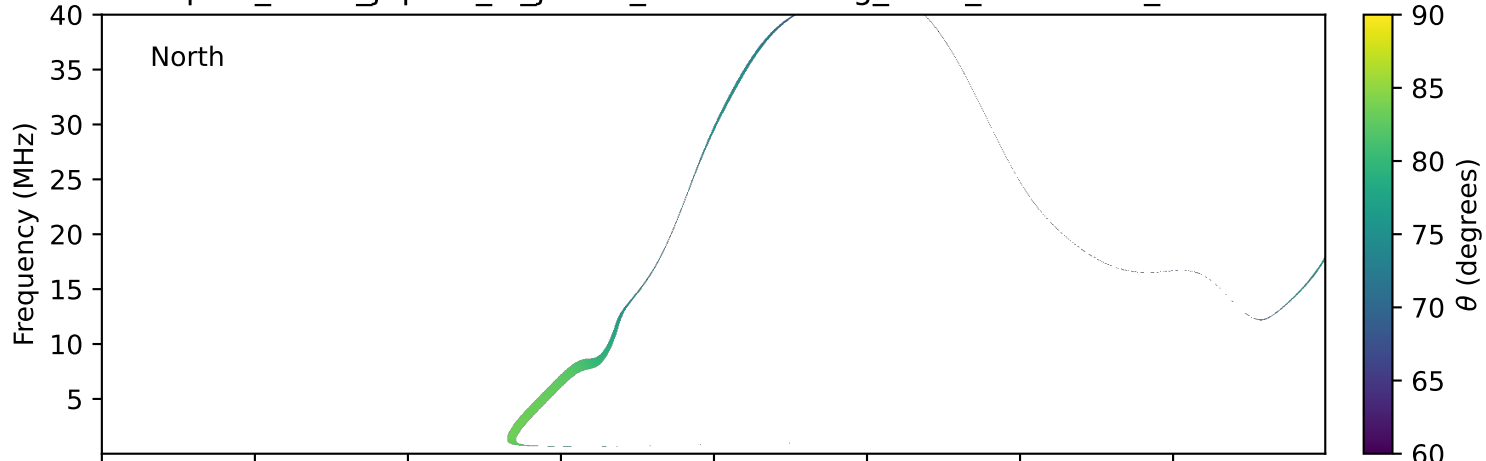
expres_earth_jupiter_io_jrm33_lossc-wid1deg_3kev_19920524_v11.cdf
