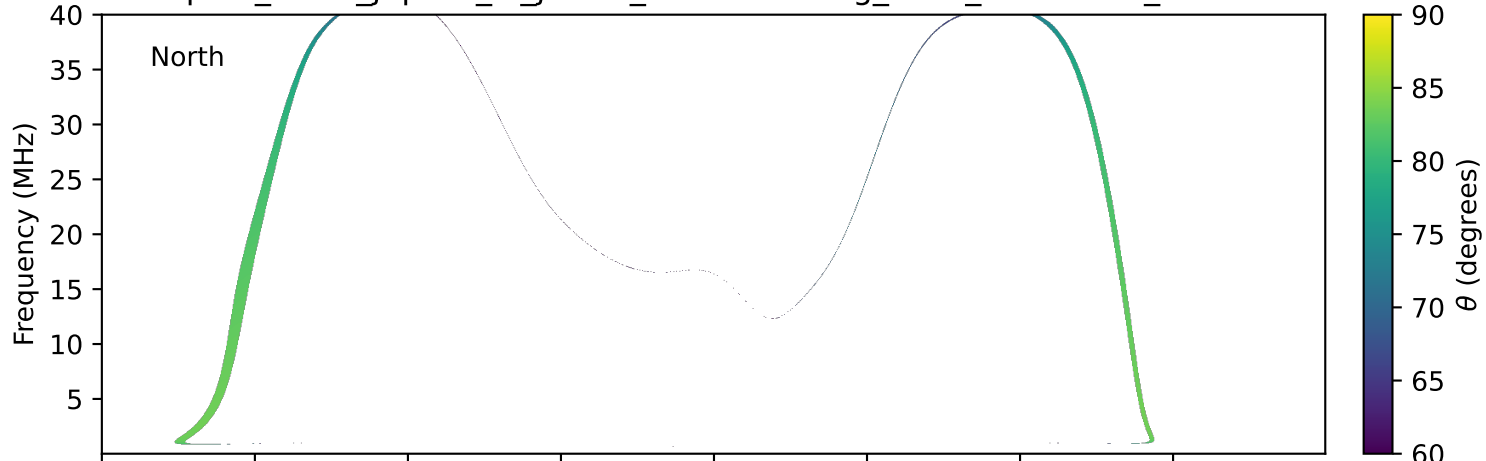
expres_earth_jupiter_io_jrm33_lossc-wid1deg_3kev_19920519_v11.cdf
