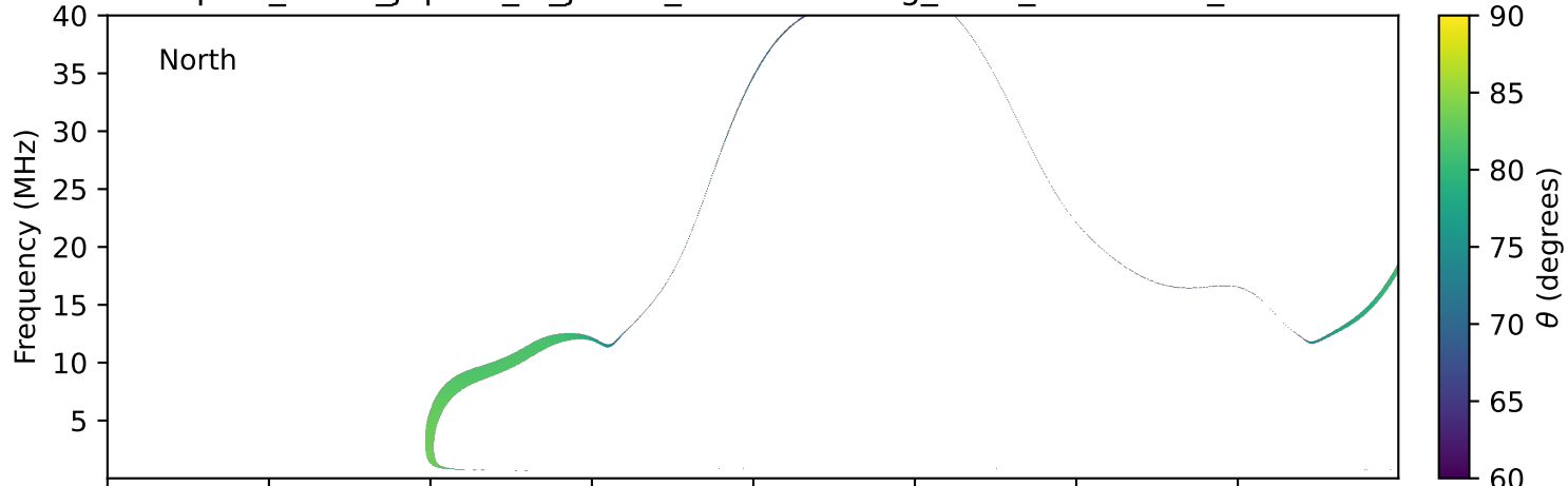
expres_earth_jupiter_io_jrm33_lossc-wid1deg_3kev_19920517_v11.cdf
