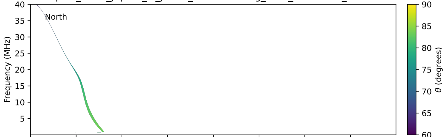
expres_earth_jupiter_io_jrm33_lossc-wid1deg_3kev_19920509_v11.cdf
