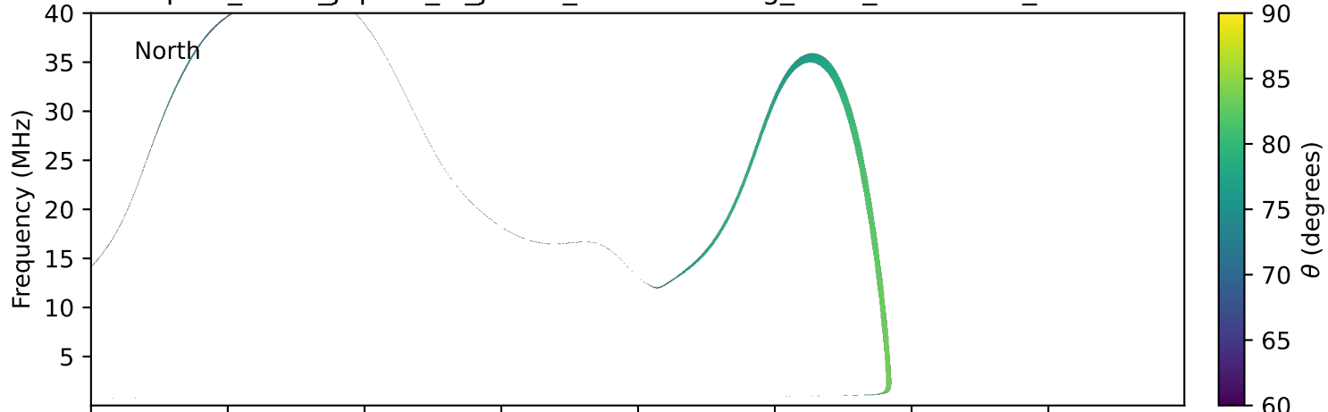
expres_earth_jupiter_io_jrm33_lossc-wid1deg_3kev_19920505_v11.cdf
