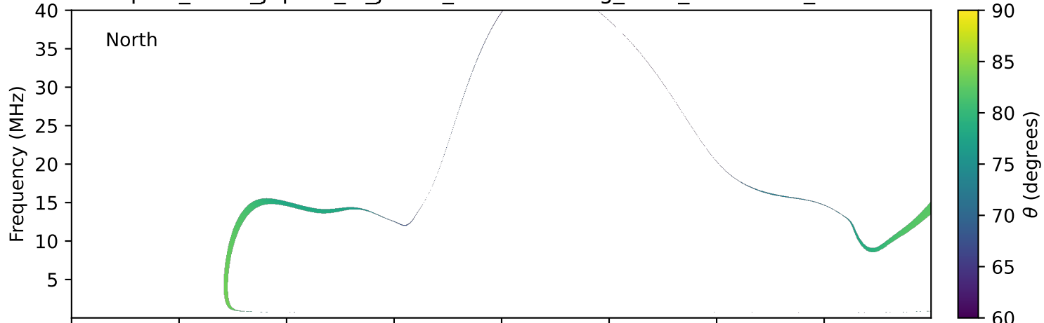
expres_earth_jupiter_io_jrm09_lossc-wid1deg_3kev_19920510_v11.cdf
