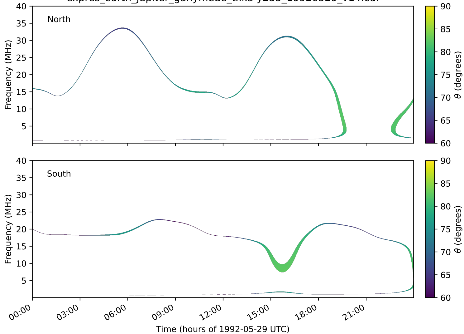
expres_earth_jupiter_ganymede_txka-y235_19920529_v14.cdf
